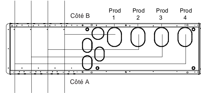
MODELES 4-4, 4-8, HS 4-4, HS 4-8
