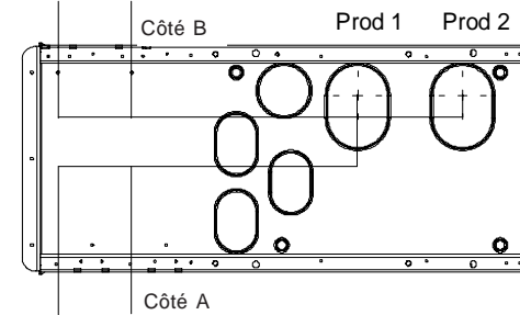
MODELES VHS 1-2 SS, VHS 2-4
