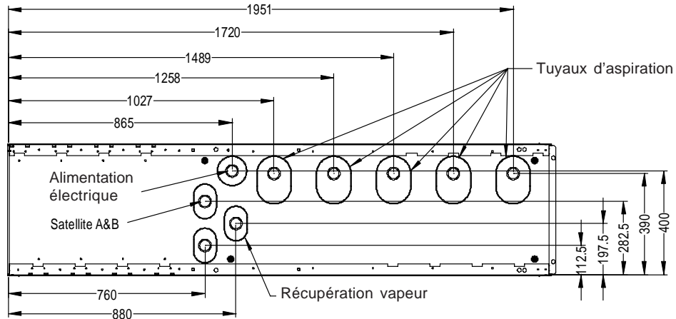
MODELES SVHSM 5-5, SVHS 5-8
